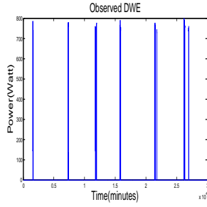
Fig. 10. Dishwasher Observed
