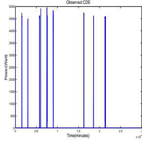
Fig. 6. Dryer Observed
