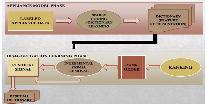
Fig. 1. Functional Overview of Our Framework
