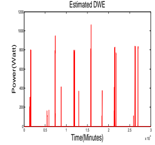
Fig. 11. Dishwasher Reconstruction
