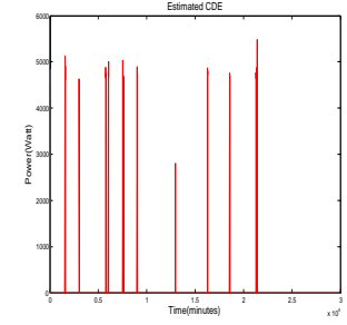
Fig. 7. Dryer Reconstruction
